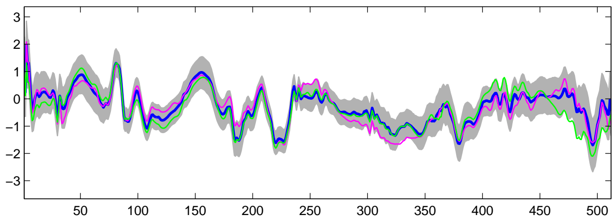
Estimated U_{15}(t) using R-WFMM: DE data, run 9
