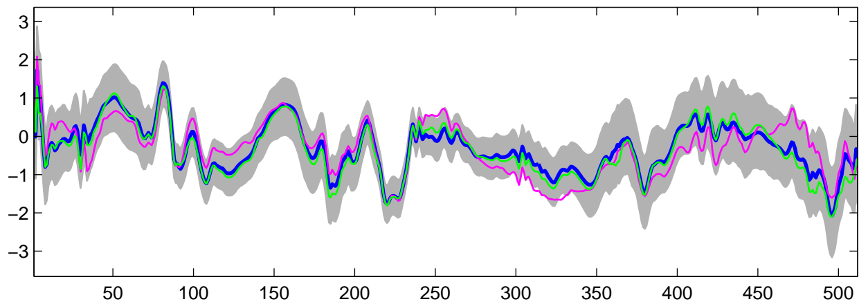
Estimated U_{15}(t) using G-WFMM: DE data, run 9
