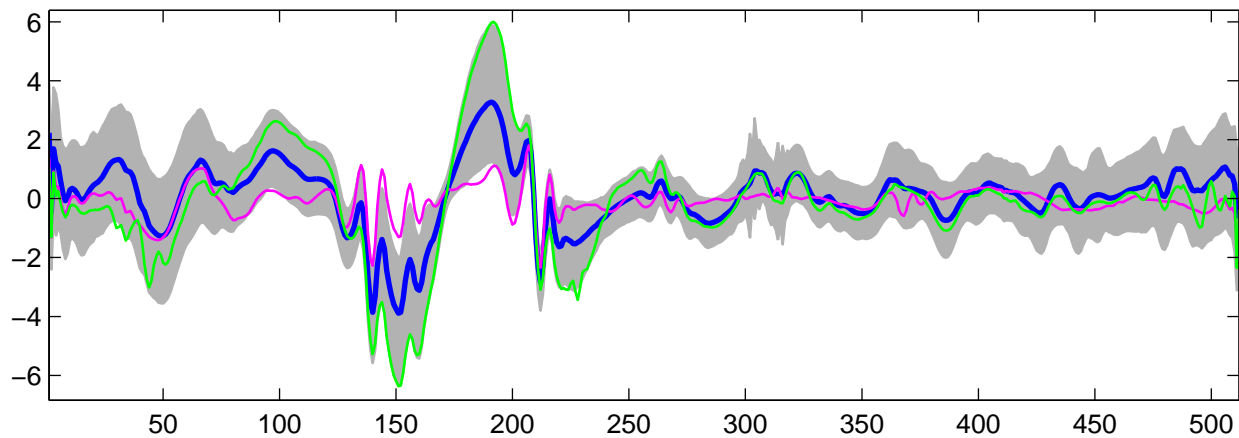
Estimated U_{15}(t) using G-WFMM: t_1 data, run 9
