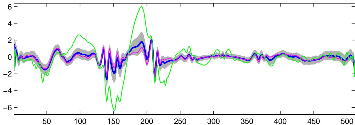
Estimated U_{15}(t) using R-WFMM: t_1 data, run 9
