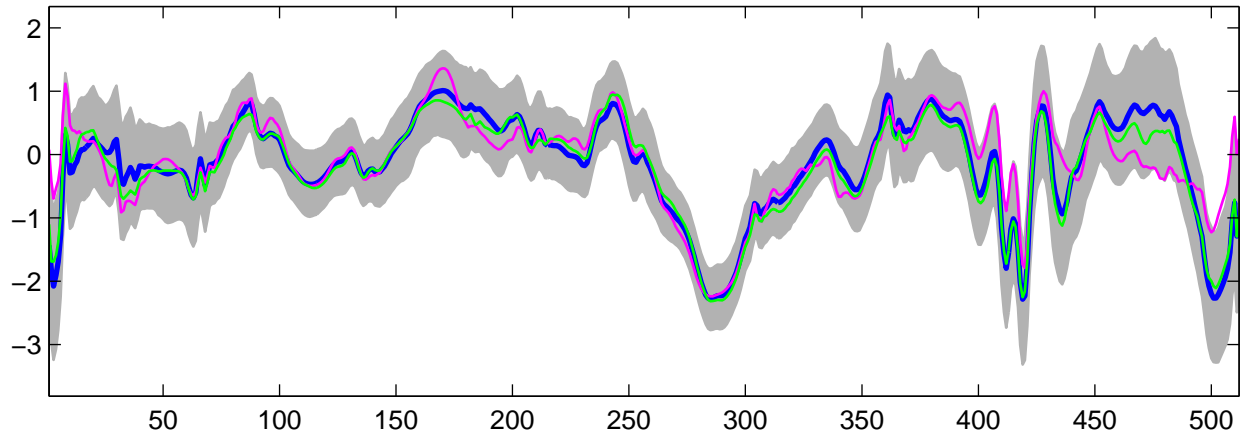
Estimated U_{15}(t) using G-WFMM: t_3 data, run 9
