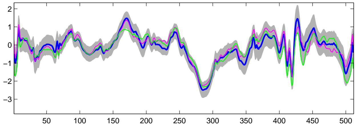
Estimated U_{15}(t) using R-WFMM: t_3 data, run 9
