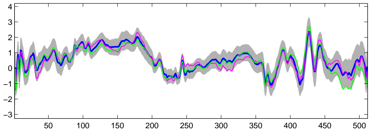
Estimated U_{16}(t) using R-WFMM: DE data, run 9
