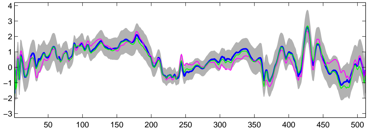
Estimated U_{16}(t) using G-WFMM: DE data, run 9
