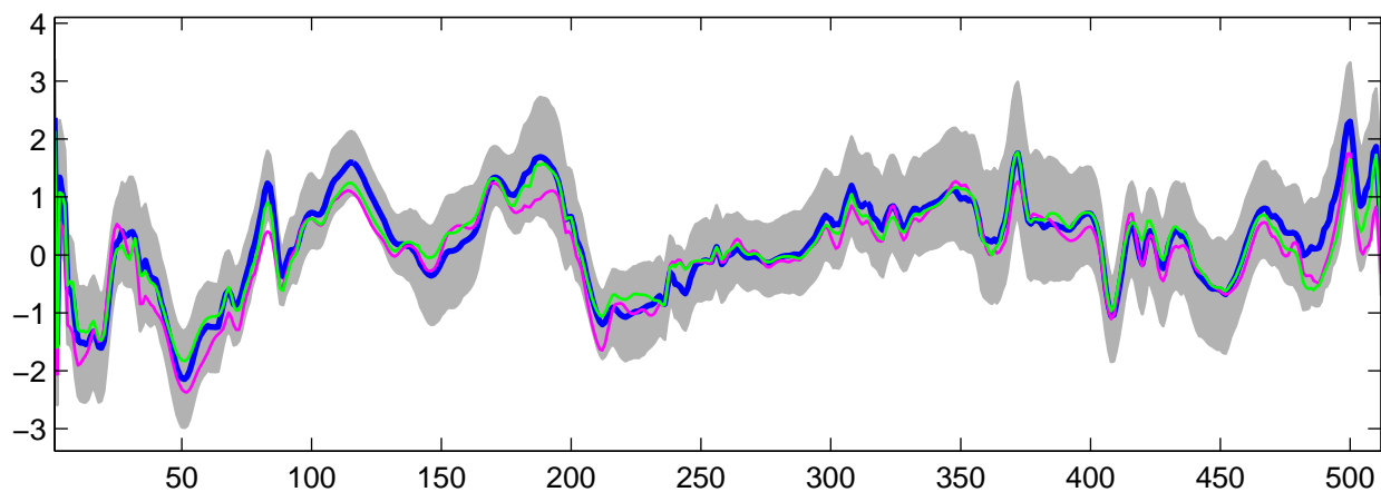
Estimated U_{16}(t) using R-WFMM: Normal data, run 9
