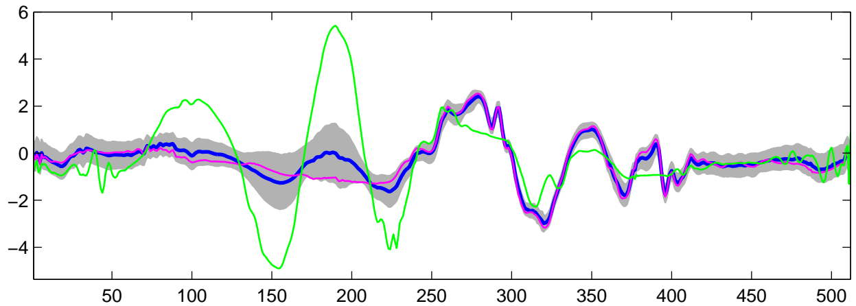
Estimated U_{16}(t) using R-WFMM: t_1 data, run 9
