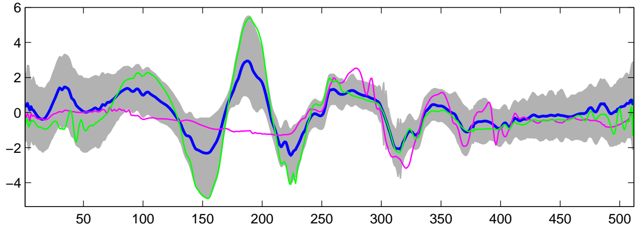
Estimated U_{16}(t) using G-WFMM: t_1 data, run 9
