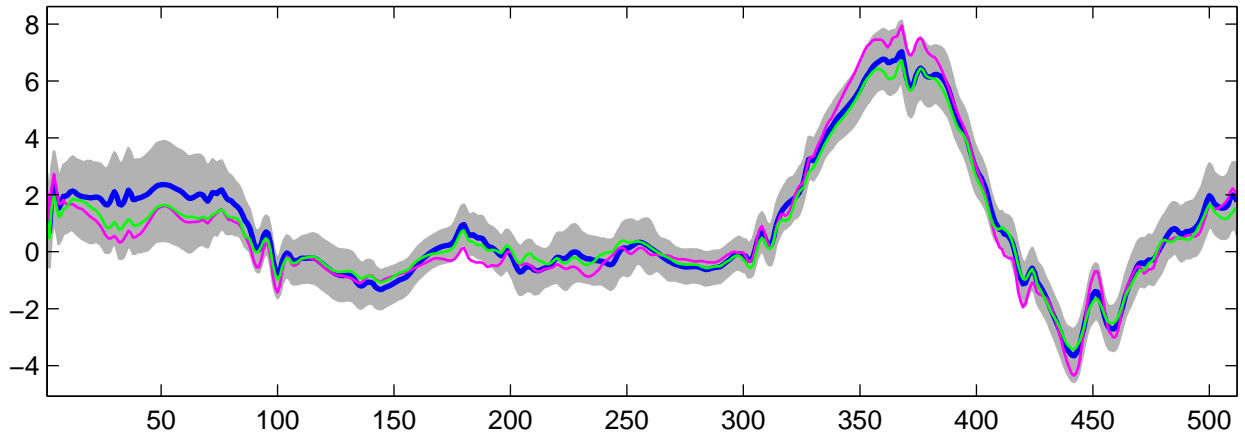
Estimated U_{16}(t) using G-WFMM: t_2 data, run 9
