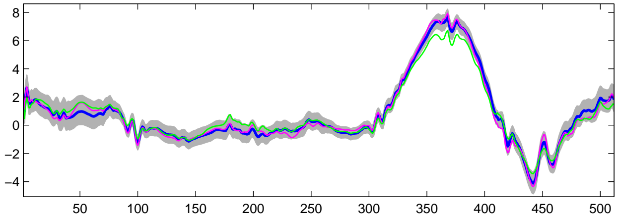
Estimated U_{16}(t) using R-WFMM: t_2 data, run 9
