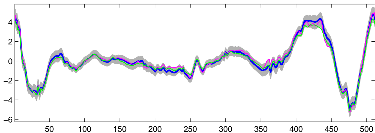
Estimated U_{16}(t) using R-WFMM: t_3 data, run 9
