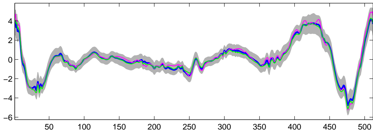
Estimated U_{16}(t) using G-WFMM: t_3 data, run 9
