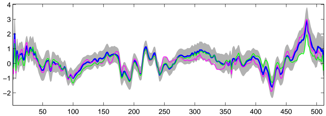
Estimated U_{17}(t) using R-WFMM: DE data, run 9
