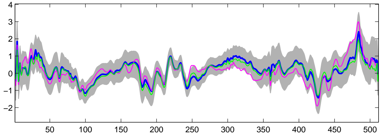
Estimated U_{17}(t) using G-WFMM: DE data, run 9
