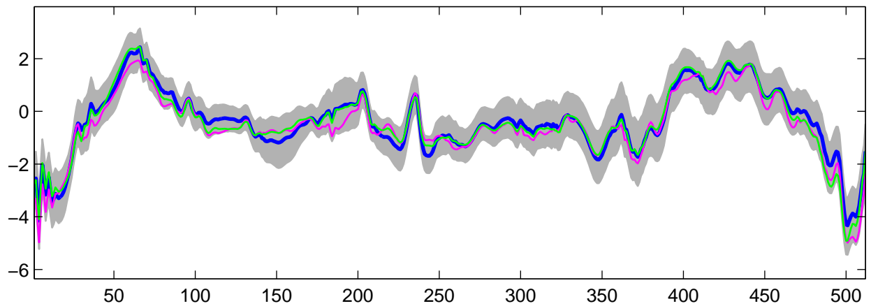
Estimated U_{17}(t) using R-WFMM: Normal data, run 9
