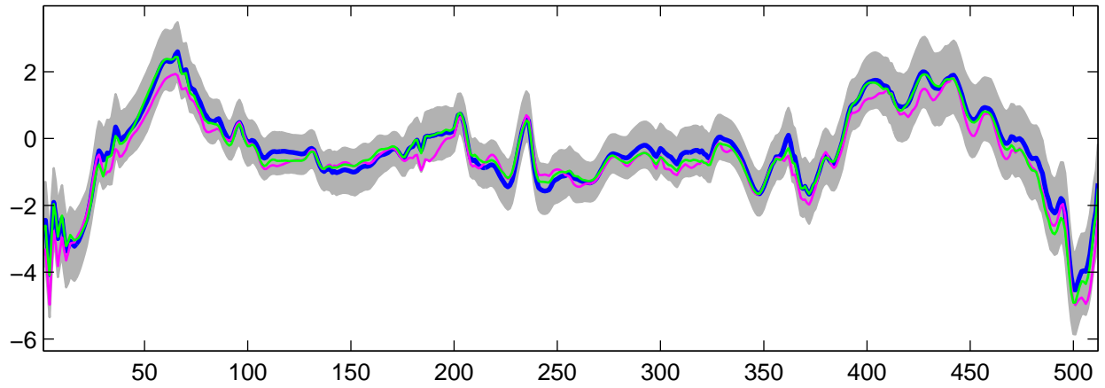
Estimated U_{17}(t) using G-WFMM: Normal data, run 9
