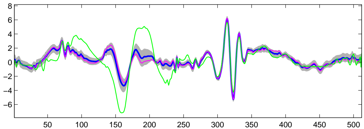
Estimated U_{17}(t) using R-WFMM: t_1 data, run 9
