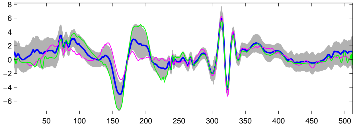
Estimated U_{17}(t) using G-WFMM: t_1 data, run 9
