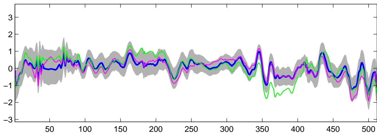
Estimated U_{17}(t) using R-WFMM: t_2 data, run 9
