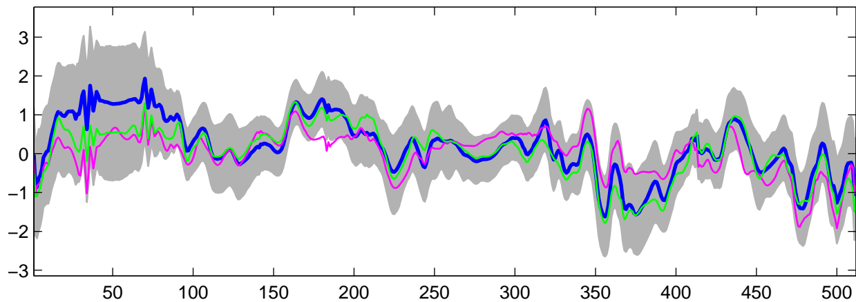
Estimated U_{17}(t) using G-WFMM: t_2 data, run 9
