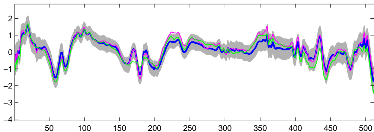
Estimated U_{17}(t) using R-WFMM: t_3 data, run 9
