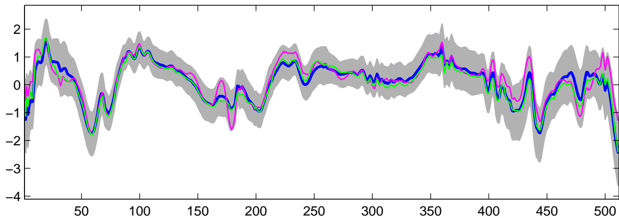
Estimated U_{17}(t) using G-WFMM: t_3 data, run 9
