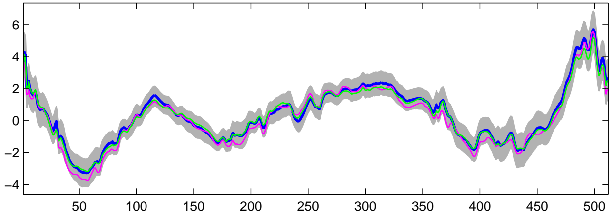
Estimated U_{18}(t) using G-WFMM: Normal data, run 9
