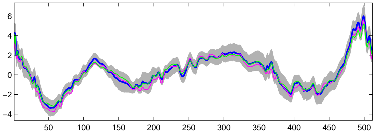
Estimated U_{18}(t) using R-WFMM: Normal data, run 9
