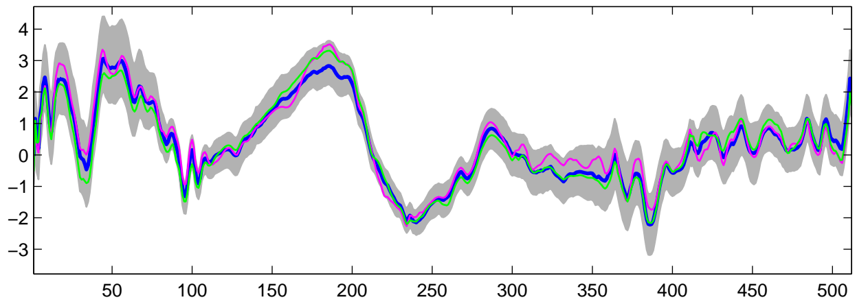
Estimated U_{19}(t) using R-WFMM: DE data, run 9
