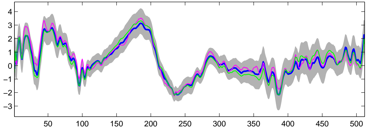
Estimated U_{19}(t) using G-WFMM: DE data, run 9
