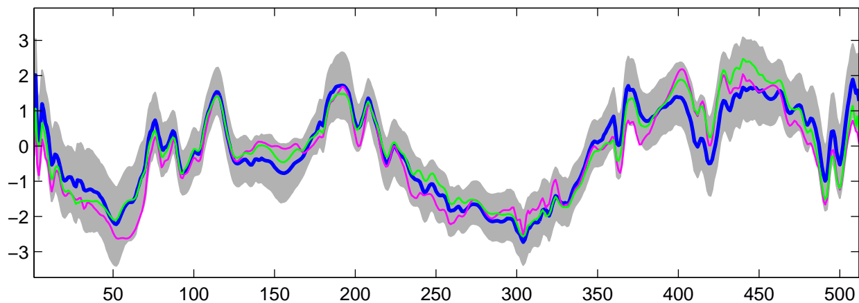
Estimated U_{19}(t) using R-WFMM: Normal data, run 9
