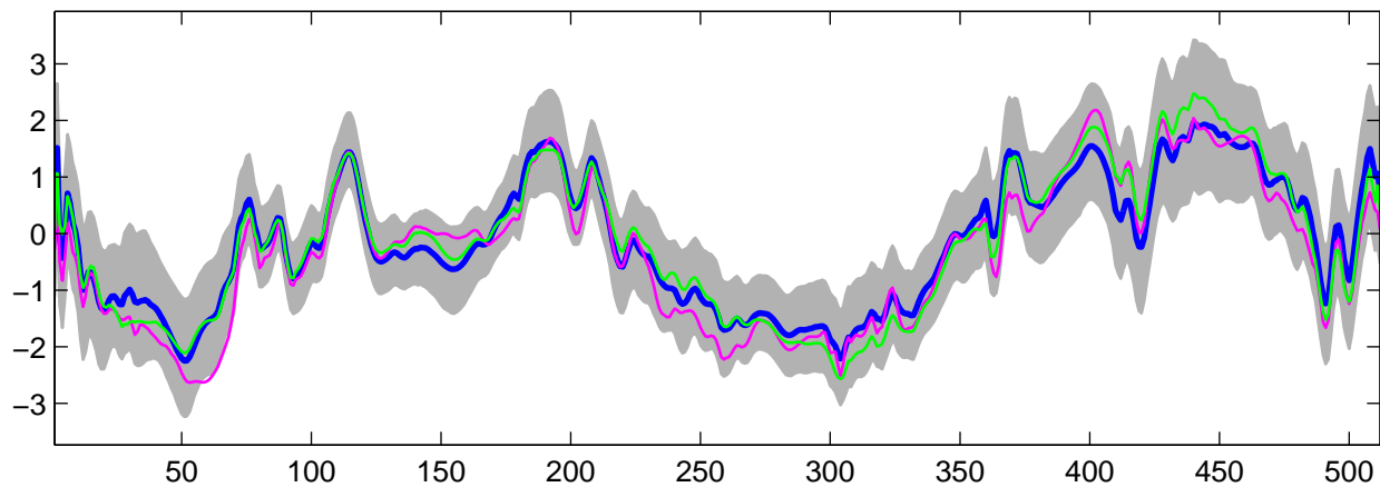
Estimated U_{19}(t) using G-WFMM: Normal data, run 9
