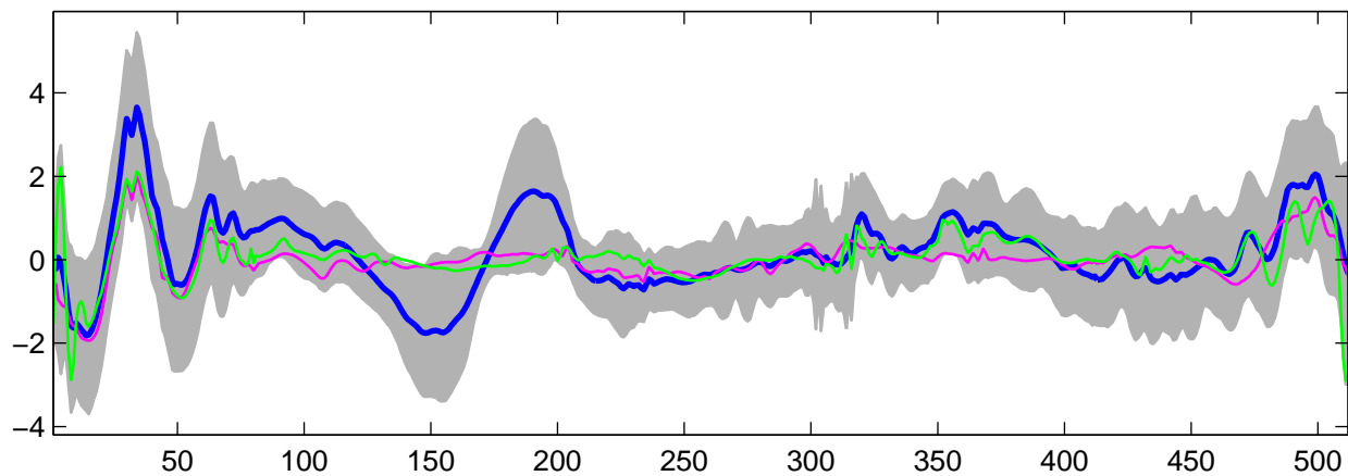
Estimated U_{19}(t) using G-WFMM: t_1 data, run 9
