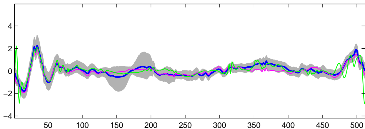
Estimated U_{19}(t) using R-WFMM: t_1 data, run 9
