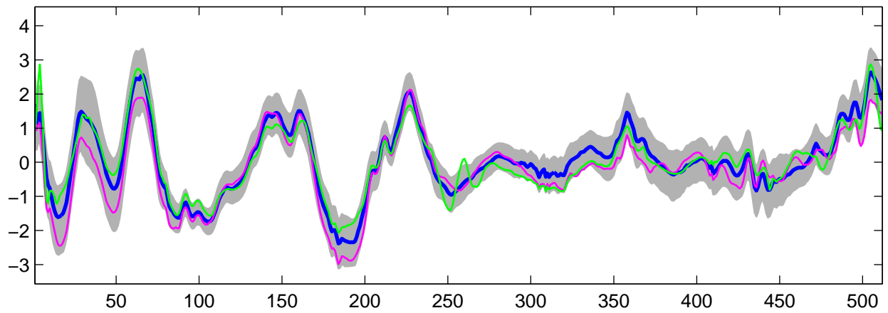
Estimated U_{19}(t) using R-WFMM: t_2 data, run 9
