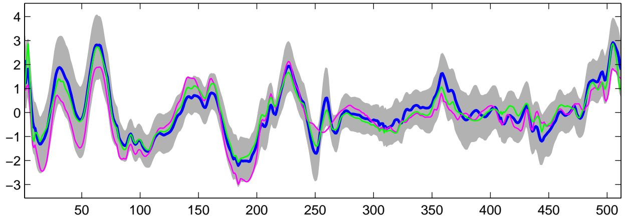
Estimated U_{19}(t) using G-WFMM: t_2 data, run 9
