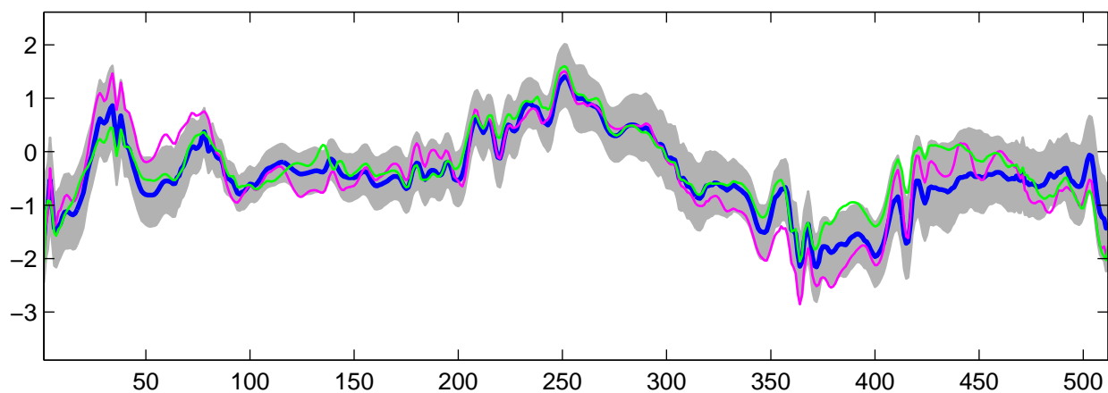
Estimated U_{19}(t) using R-WFMM: t_3 data, run 9
