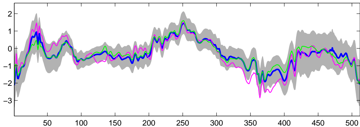
Estimated U_{19}(t) using G-WFMM: t_3 data, run 9
