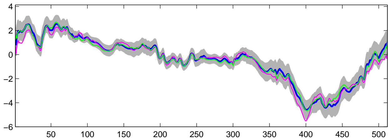
Estimated U_1(t) using R-WFMM: DE data, run 9
