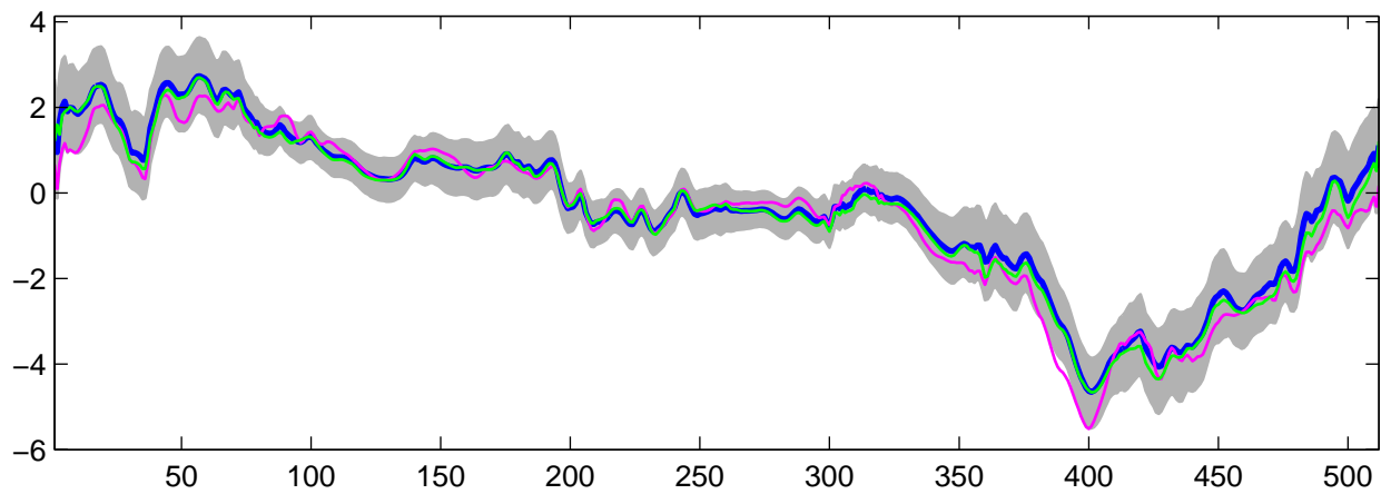
Estimated U_1(t) using G-WFMM: DE data, run 9
