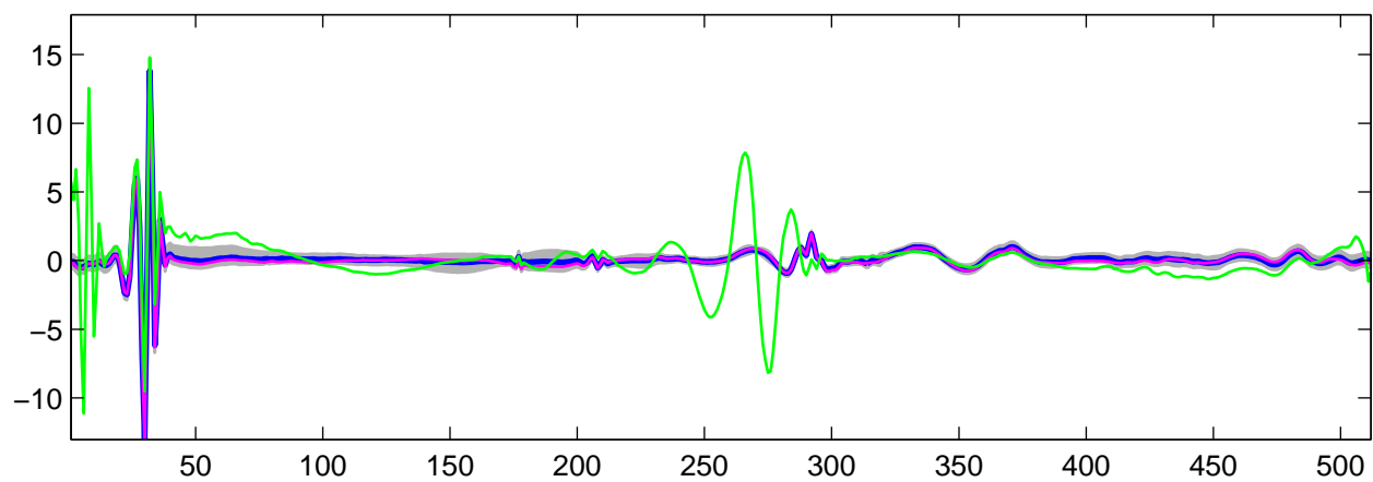
Estimated U_1(t) using R-WFMM: t_1 data, run 9
