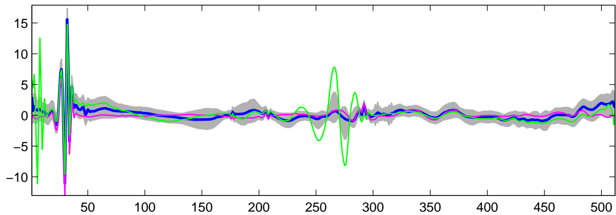
Estimated U_1(t) using G-WFMM: t_1 data, run 9
