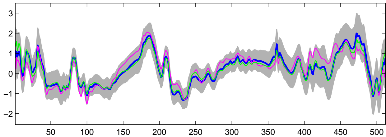
Estimated U_1(t) using G-WFMM: t_3 data, run 9
