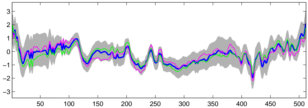
Estimated U_{20}(t) using R-WFMM: DE data, run 9
