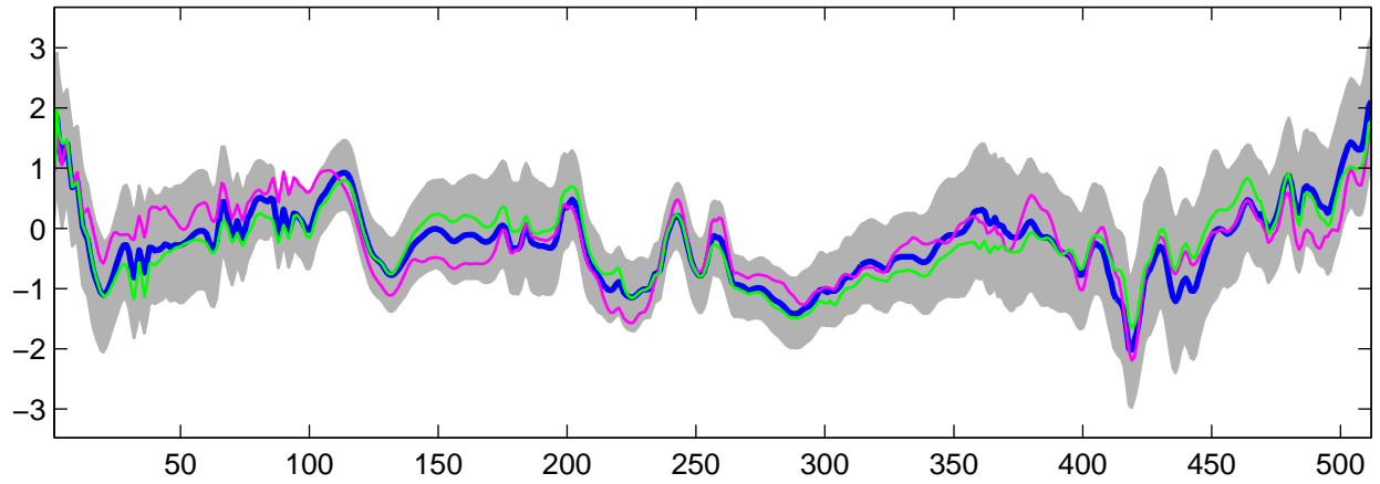
Estimated U_{20}(t) using G-WFMM: DE data, run 9
