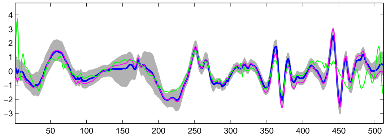
Estimated U_{20}(t) using R-WFMM: t_1 data, run 9
