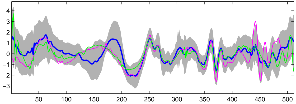
Estimated U_{20}(t) using G-WFMM: t_1 data, run 9
