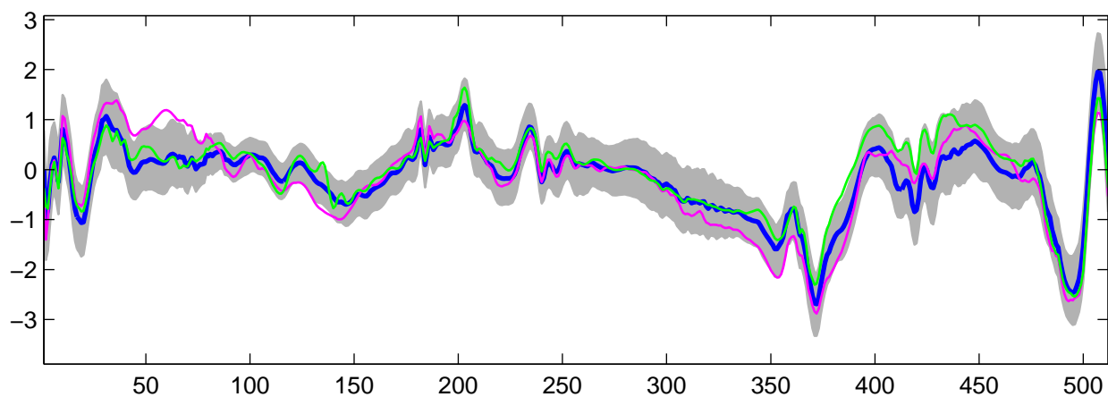
Estimated U_{20}(t) using R-WFMM: t_3 data, run 9
