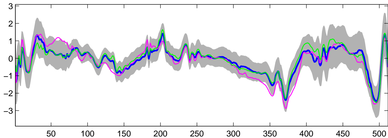
Estimated U_{20}(t) using G-WFMM: t_3 data, run 9
