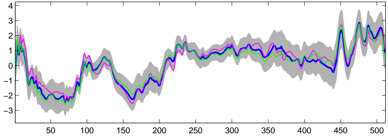
Estimated U_{21}(t) using G-WFMM: DE data, run 9
