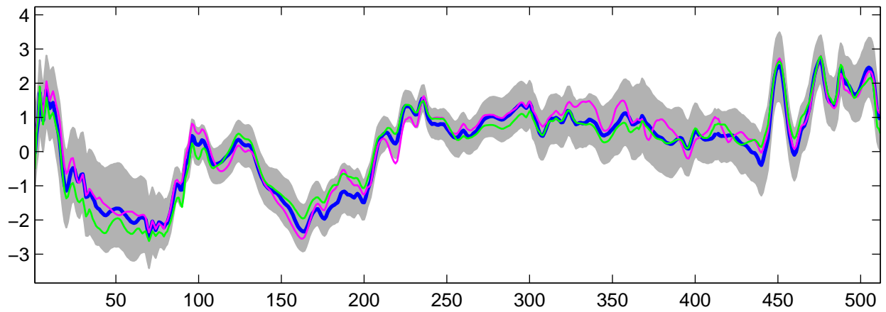
Estimated U_{21}(t) using R-WFMM: DE data, run 9
