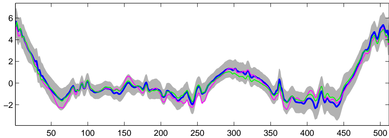
Estimated U_{21}(t) using G-WFMM: Normal data, run 9
