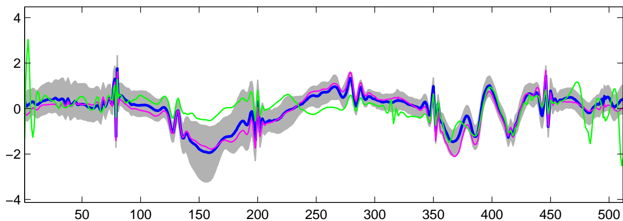
Estimated U_{21}(t) using R-WFMM: t_1 data, run 9
