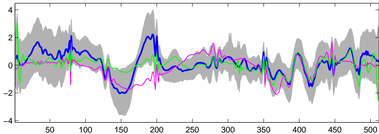
Estimated U_{21}(t) using G-WFMM: t_1 data, run 9
