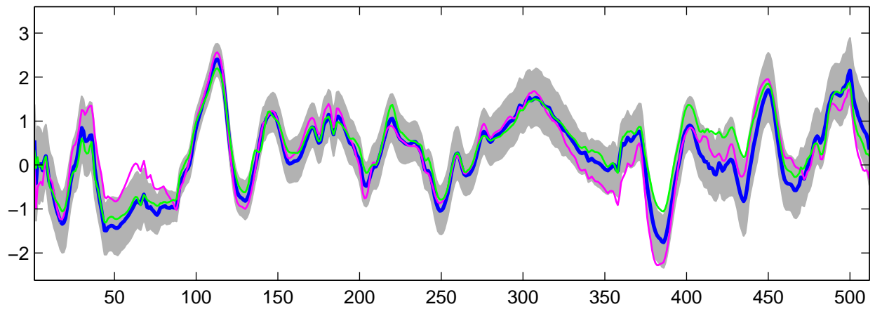
Estimated U_{21}(t) using R-WFMM: t_3 data, run 9
