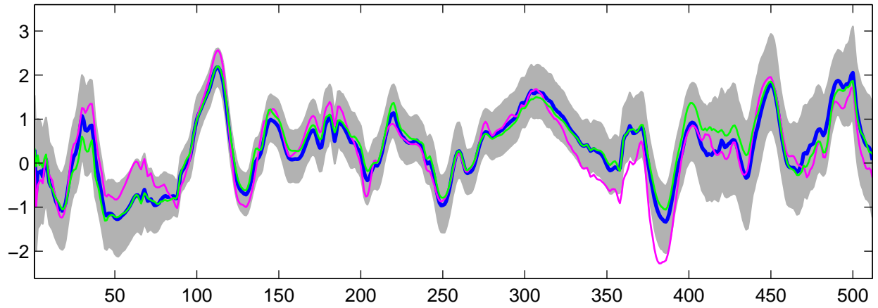
Estimated U_{21}(t) using G-WFMM: t_3 data, run 9
