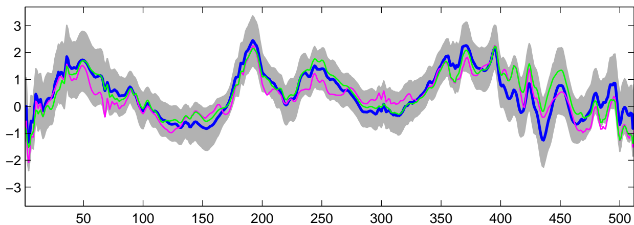
Estimated U_{22}(t) using R-WFMM: Normal data, run 9
