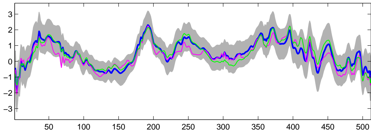
Estimated U_{22}(t) using G-WFMM: Normal data, run 9
