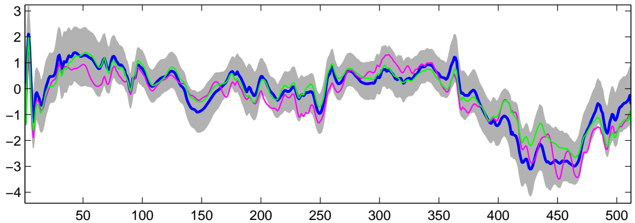
Estimated U_{23}(t) using R-WFMM: Normal data, run 9
