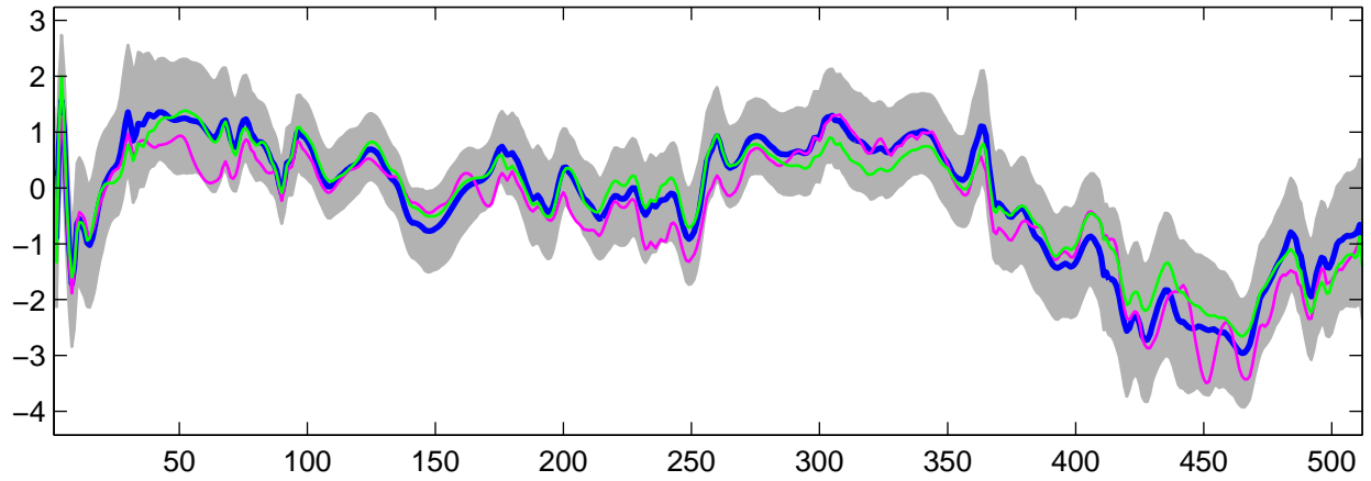
Estimated U_{23}(t) using G-WFMM: Normal data, run 9
