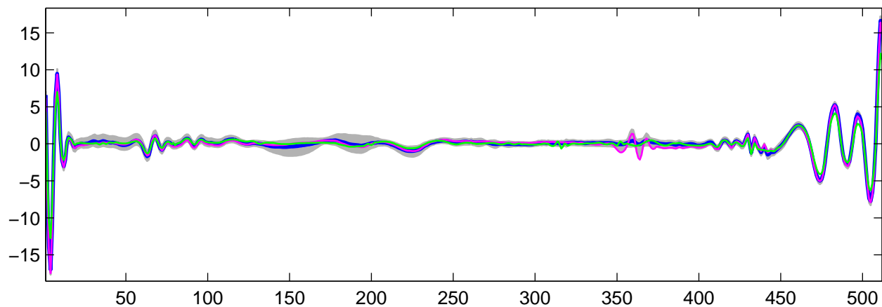
Estimated U_{23}(t) using R-WFMM: t_1 data, run 9
