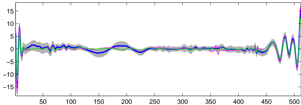
Estimated U_{23}(t) using G-WFMM: t_1 data, run 9
