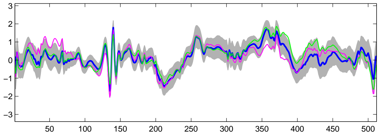
Estimated U_{23}(t) using R-WFMM: t_3 data, run 9
