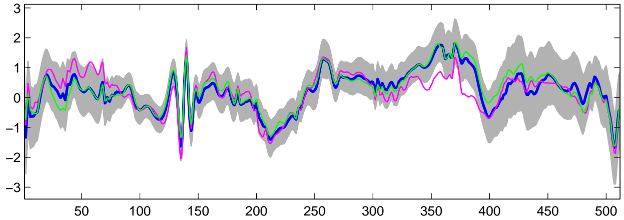
Estimated U_{23}(t) using G-WFMM: t_3 data, run 9
