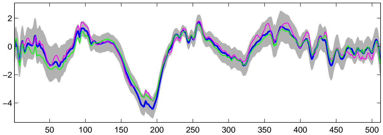
Estimated U_{24}(t) using R-WFMM: DE data, run 9
