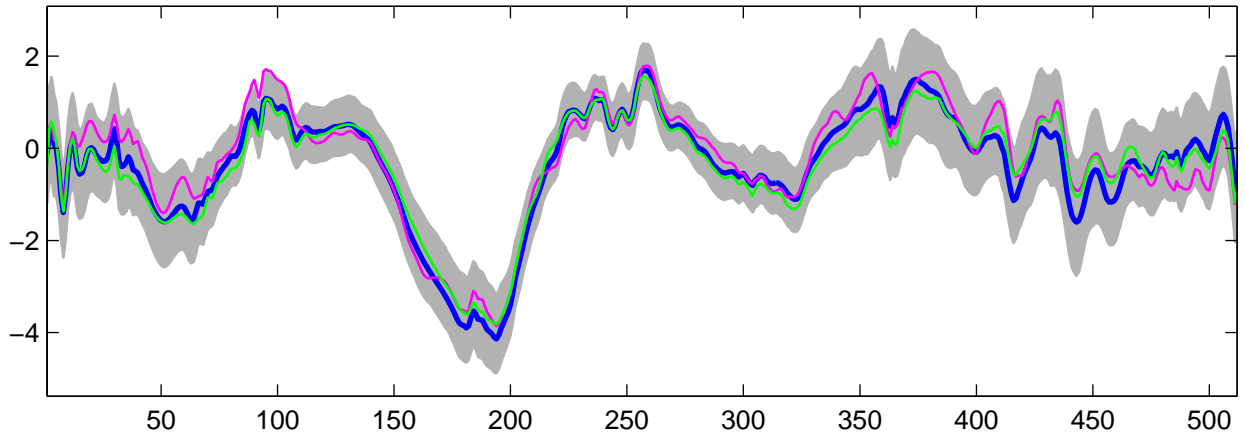
Estimated U_{24}(t) using G-WFMM: DE data, run 9
