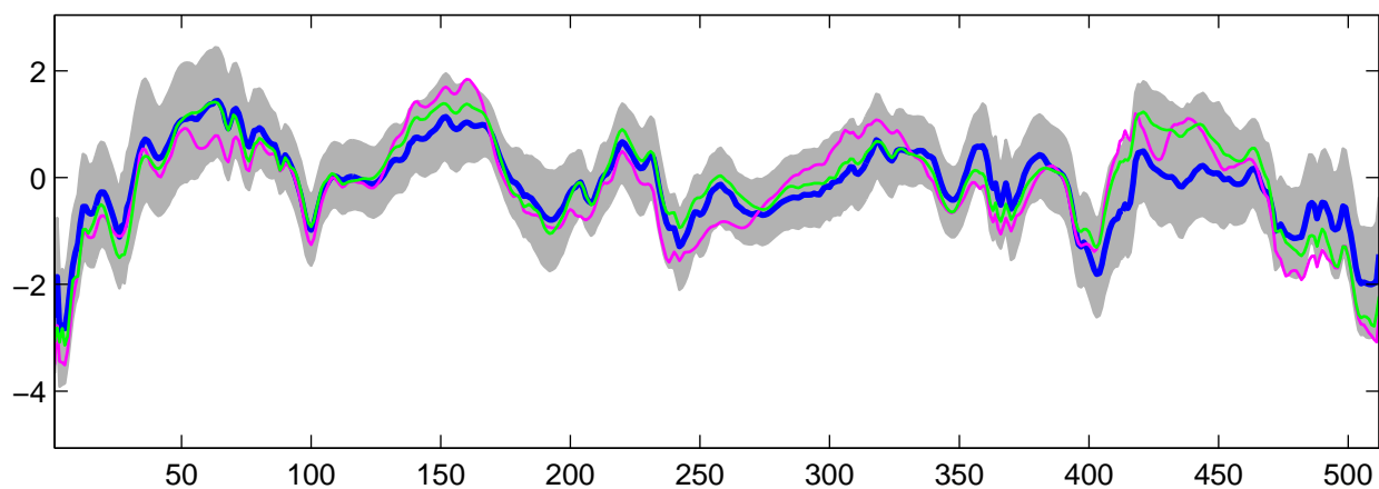
Estimated U_{24}(t) using R-WFMM: Normal data, run 9
