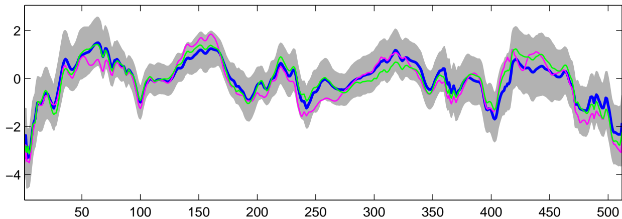
Estimated U_{24}(t) using G-WFMM: Normal data, run 9
