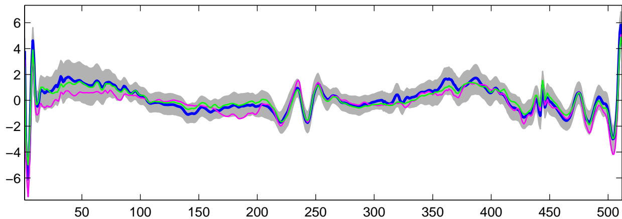
Estimated U_{24}(t) using G-WFMM: t_2 data, run 9
