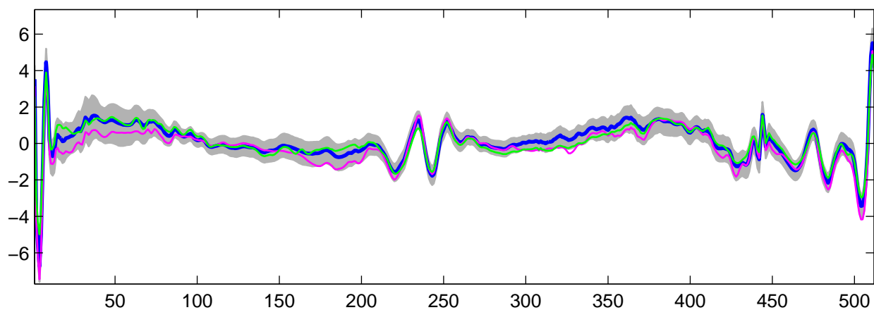
Estimated U_{24}(t) using R-WFMM: t_2 data, run 9
