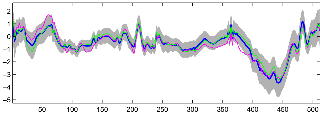
Estimated U_{24}(t) using G-WFMM: t_3 data, run 9
