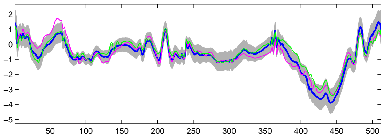
Estimated U_{24}(t) using R-WFMM: t_3 data, run 9
