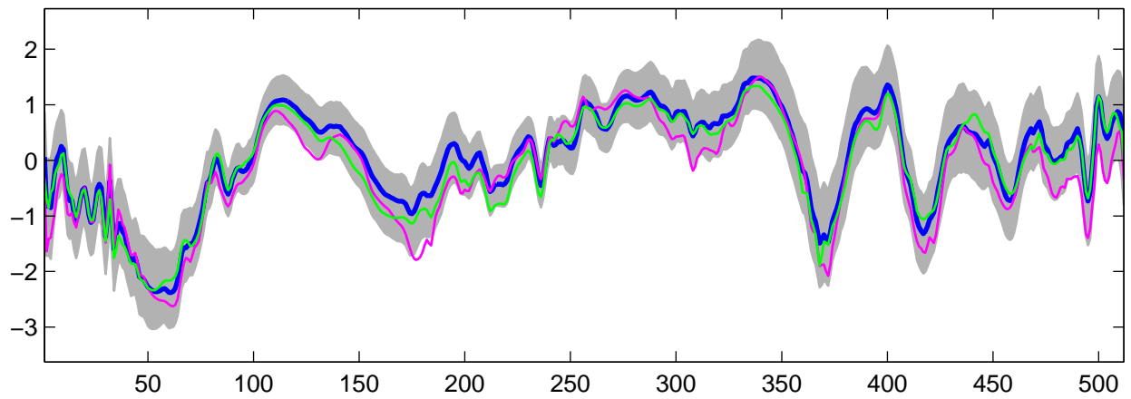
Estimated U_{25}(t) using R-WFMM: DE data, run 9
