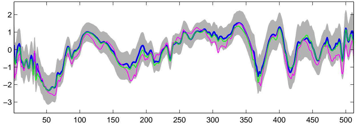
Estimated U_{25}(t) using G-WFMM: DE data, run 9
