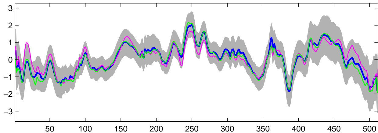
Estimated U_{25}(t) using G-WFMM: Normal data, run 9
