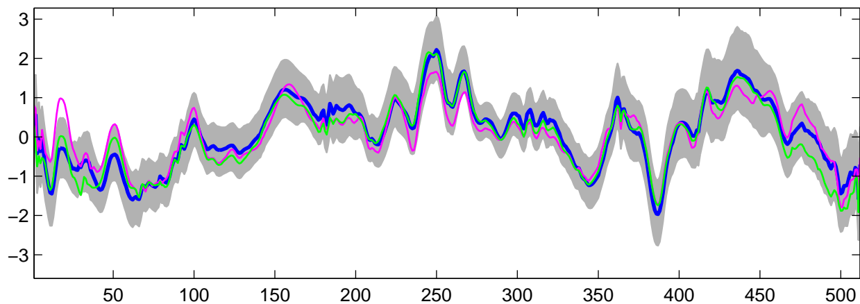
Estimated U_{25}(t) using R-WFMM: Normal data, run 9
