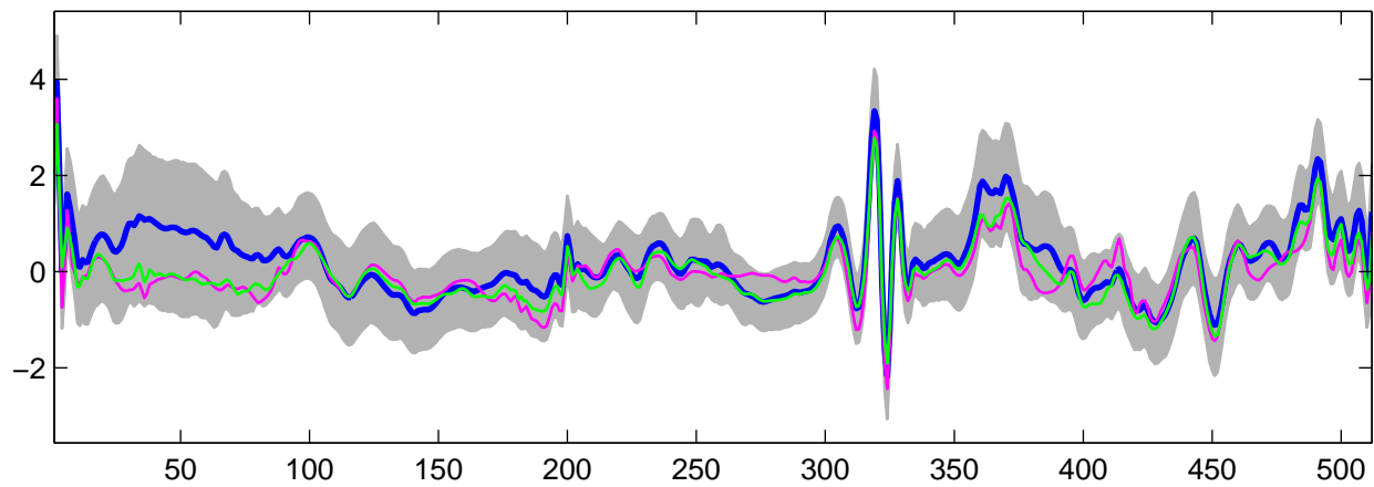
Estimated U_{25}(t) using G-WFMM: t_2 data, run 9
