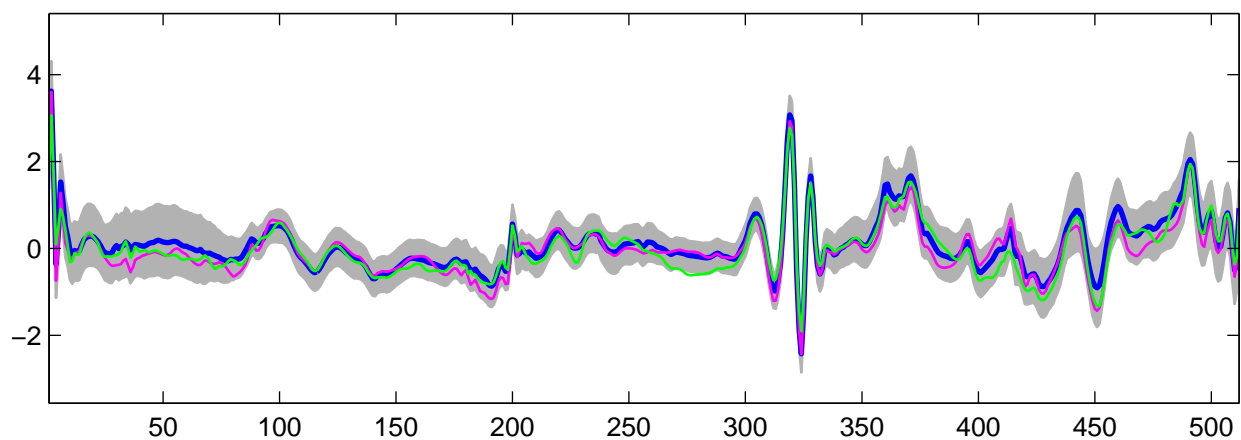
Estimated U_{25}(t) using R-WFMM: t_2 data, run 9
