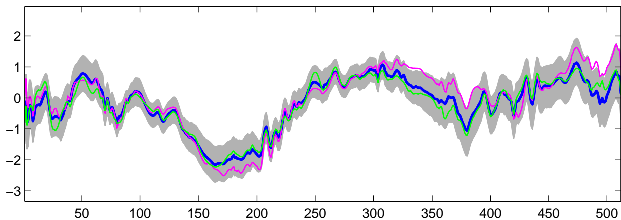
Estimated U_{25}(t) using R-WFMM: t_3 data, run 9
