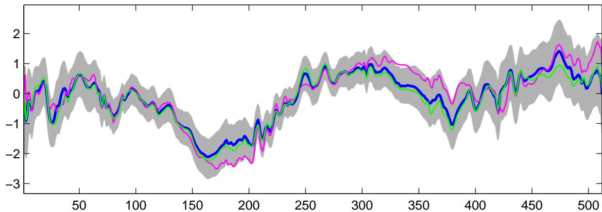
Estimated U_{25}(t) using G-WFMM: t_3 data, run 9
