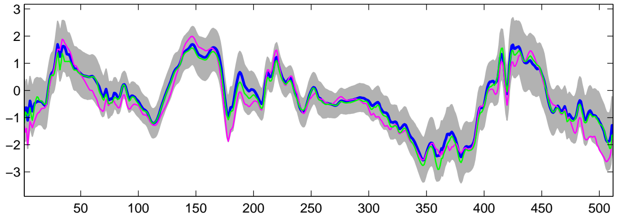
Estimated U_{26}(t) using G-WFMM: DE data, run 9
