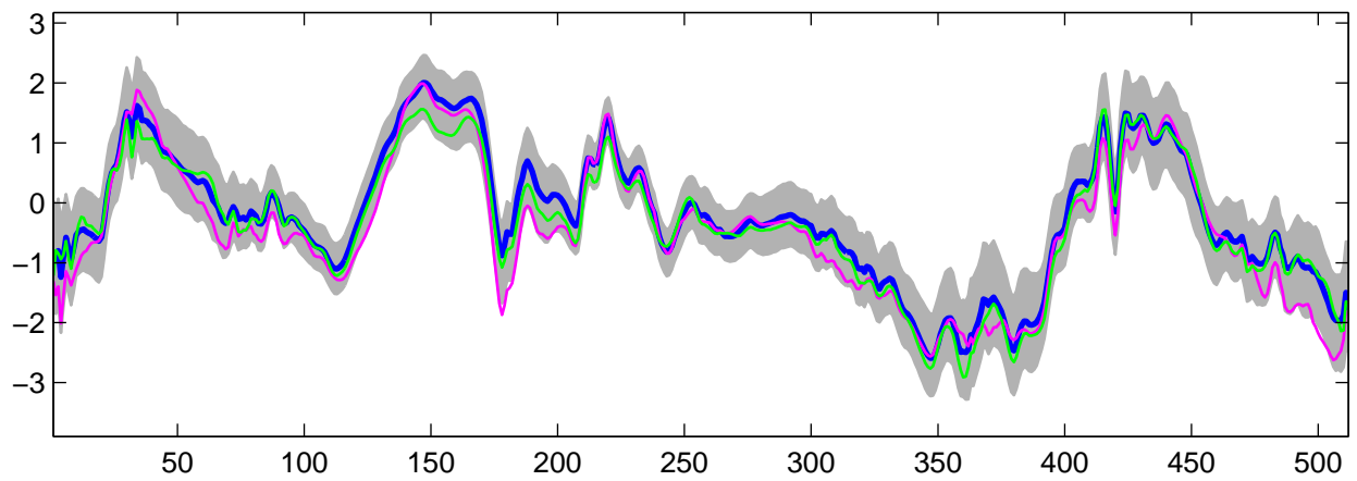
Estimated U_{26}(t) using R-WFMM: DE data, run 9
