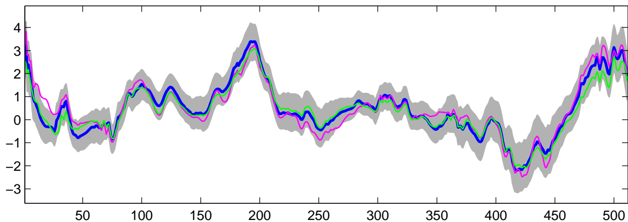
Estimated U_{26}(t) using R-WFMM: Normal data, run 9
