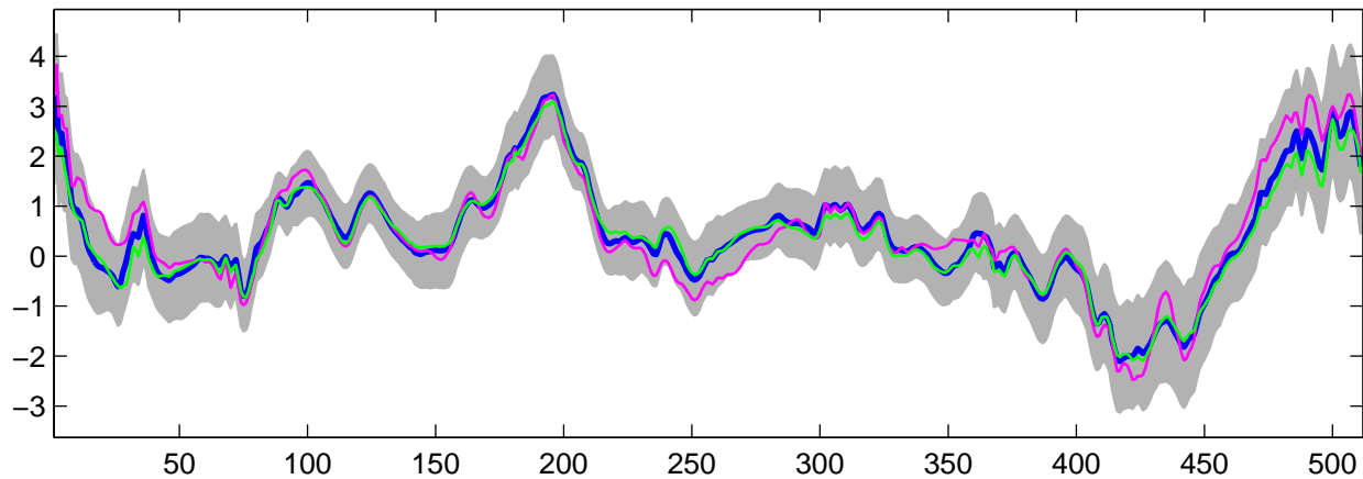
Estimated U_{26}(t) using G-WFMM: Normal data, run 9
