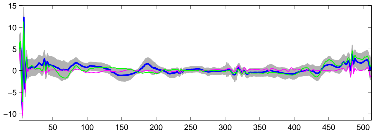
Estimated U_{26}(t) using G-WFMM: t_1 data, run 9
