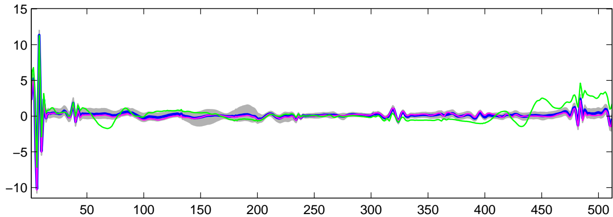
Estimated U_{26}(t) using R-WFMM: t_1 data, run 9
