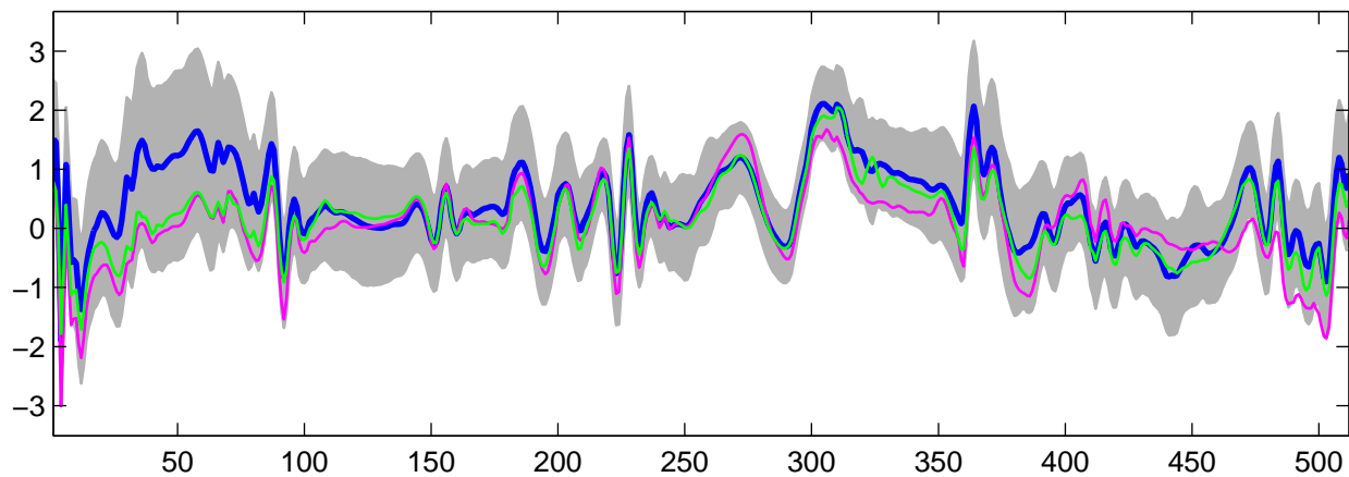
Estimated U_{26}(t) using G-WFMM: t_2 data, run 9
