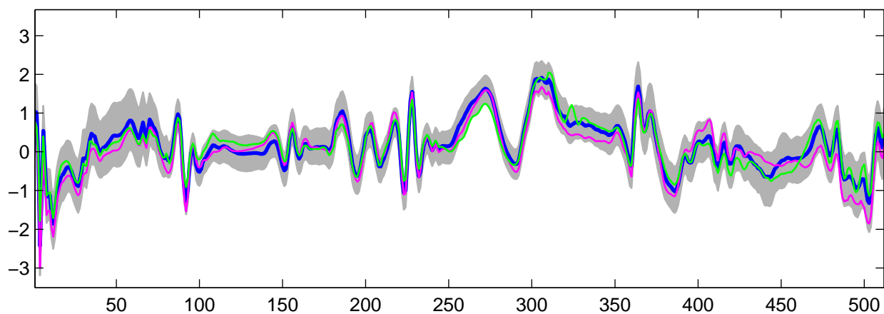
Estimated U_{26}(t) using R-WFMM: t_2 data, run 9
