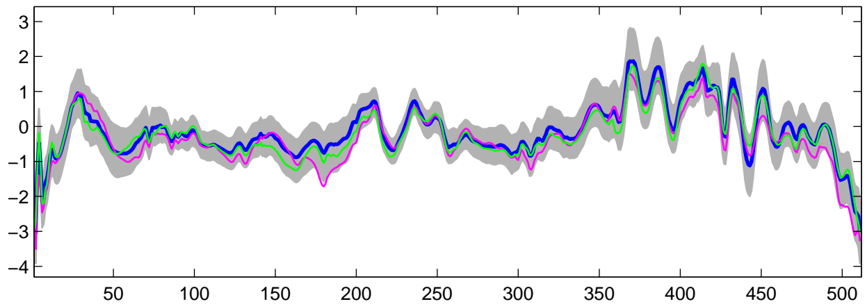
Estimated U_{27}(t) using R-WFMM: DE data, run 9
