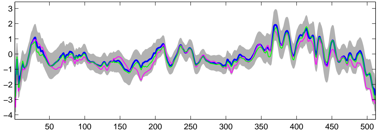
Estimated U_{27}(t) using G-WFMM: DE data, run 9
