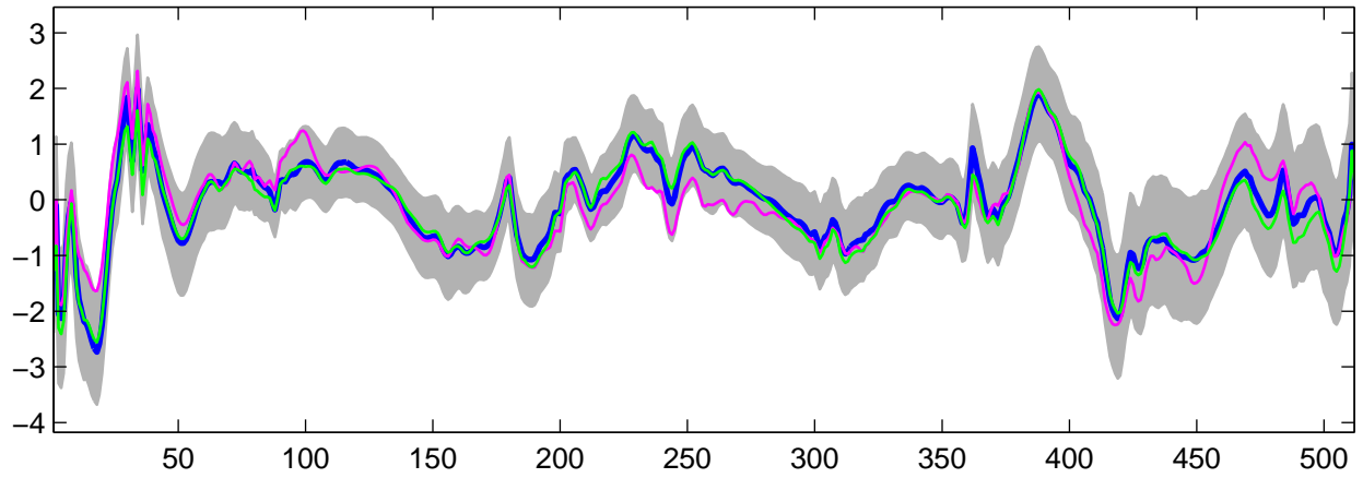
Estimated U_{27}(t) using G-WFMM: Normal data, run 9
