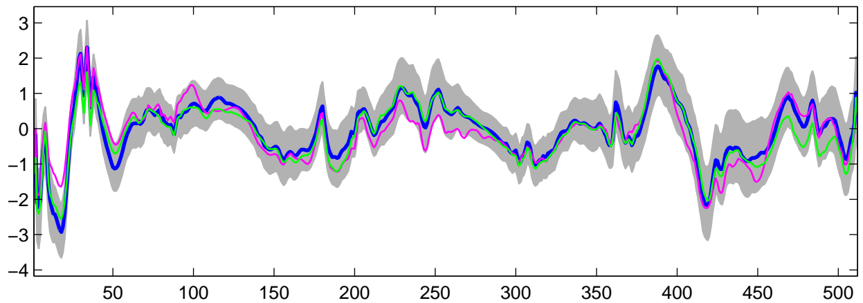
Estimated U_{27}(t) using R-WFMM: Normal data, run 9
