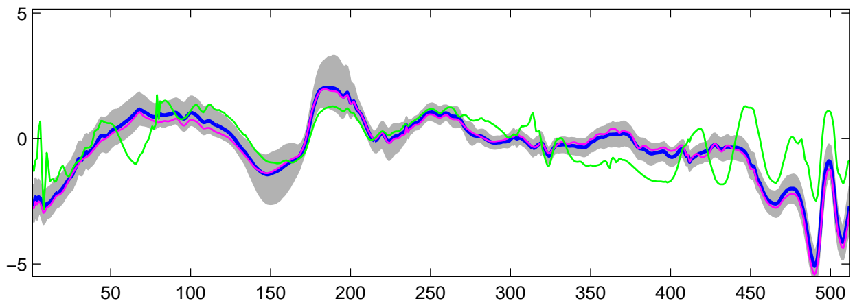
Estimated U_{27}(t) using R-WFMM: t_1 data, run 9
