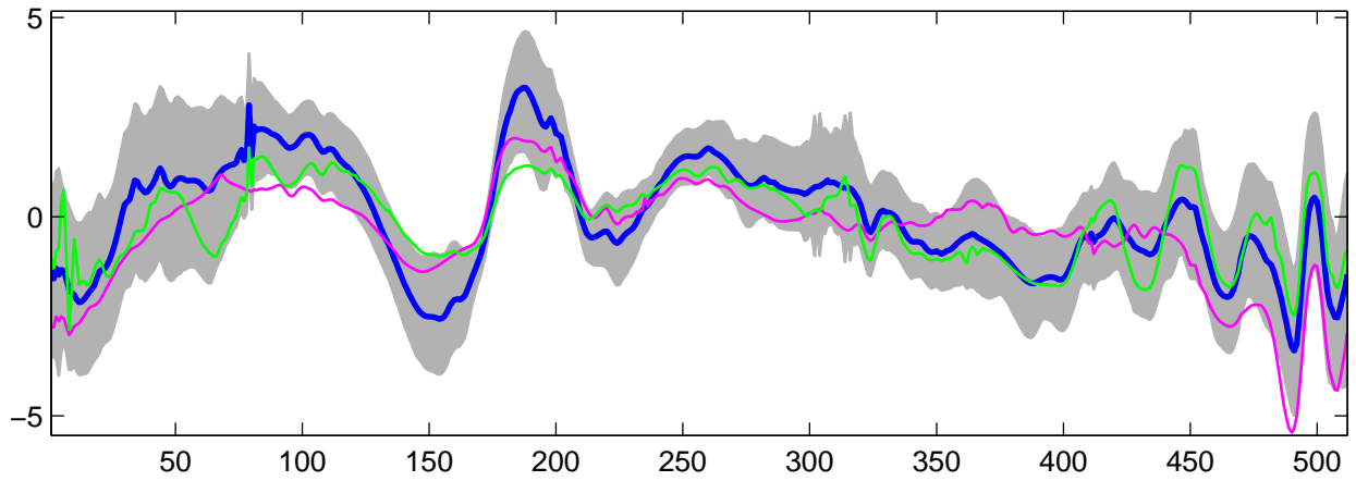
Estimated U_{27}(t) using G-WFMM: t_1 data, run 9
