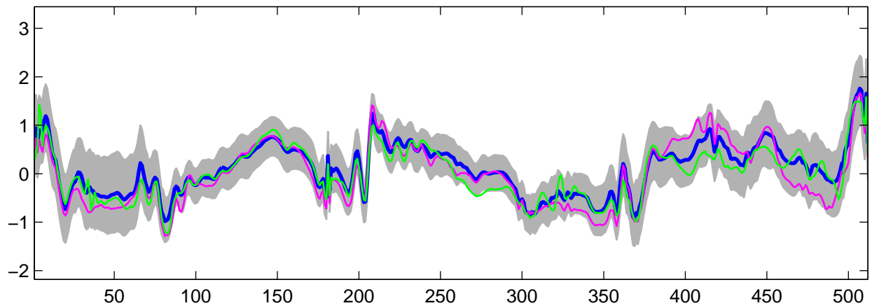
Estimated U_{27}(t) using R-WFMM: t_2 data, run 9
