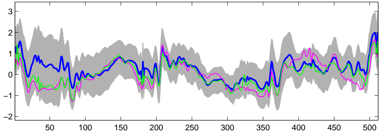
Estimated U_{27}(t) using G-WFMM: t_2 data, run 9
