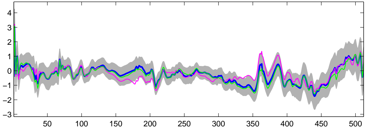
Estimated U_{27}(t) using G-WFMM: t_3 data, run 9
