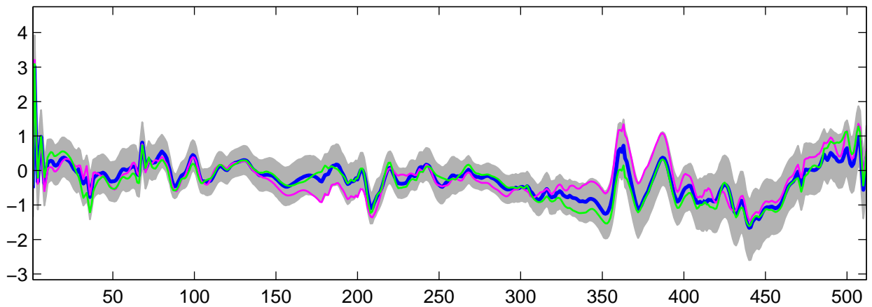
Estimated U_{27}(t) using R-WFMM: t_3 data, run 9
